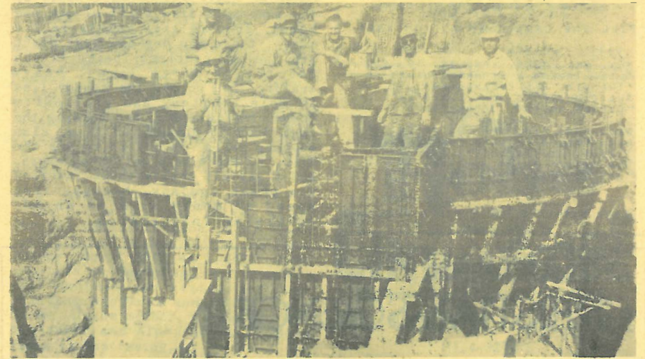
NEW SEWER DIGESTOR SHAPES UP AS WORKMEN INSTALL MOVING PARTS IN HUGE CONCRETE PLANT. STILL WITHIN UNIQUE STEEL FORMS. CONTRACTOR E. P. WATSON SAYS IT SHOULD BE RUNNING BY MAY 15. HIS MEN PICTURED: (L TO R): WALT PARKER, (IN CAP), FOREMAN; ABOVE HIM, NOT KNOWN; BOB GEERING; (UNKNOWN, IN CAP); A. L. FRYE, CLYDE LEHMAN AND JIM GEERING. - IRVINE PHOTO.
